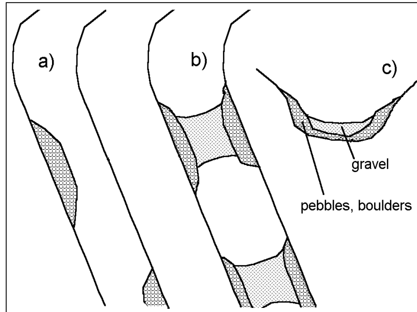
Fig. 5: Induction of turbulence (a) and establishment of spawning grounds (b) from above, c) cross section).
